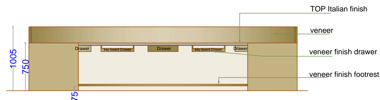
Elevation-B
